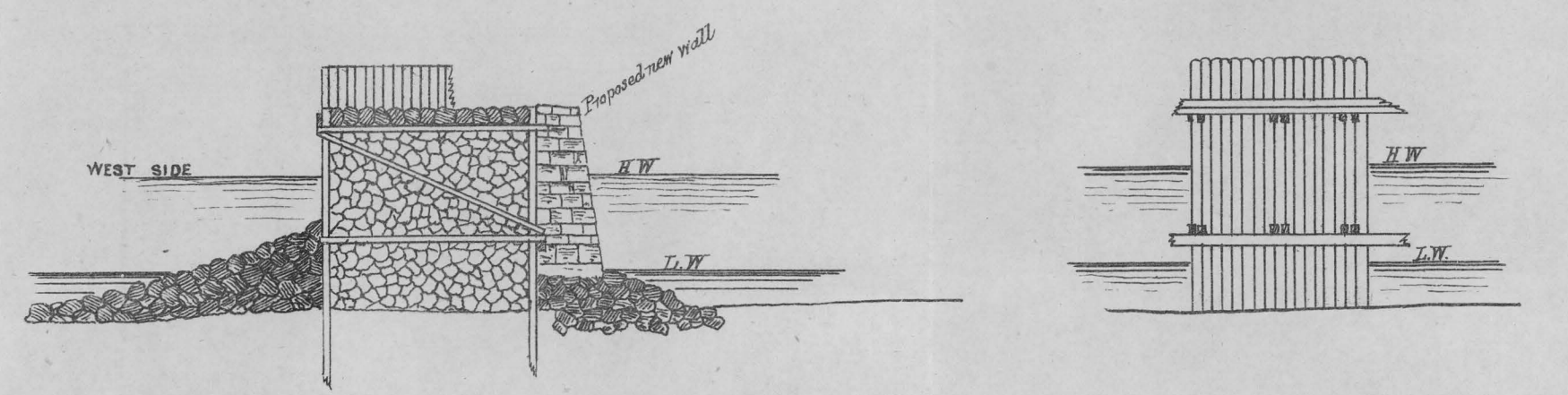
— EXTENSION OF BREAKWATER — Stone slopes & walls to be added when piles are worn away
