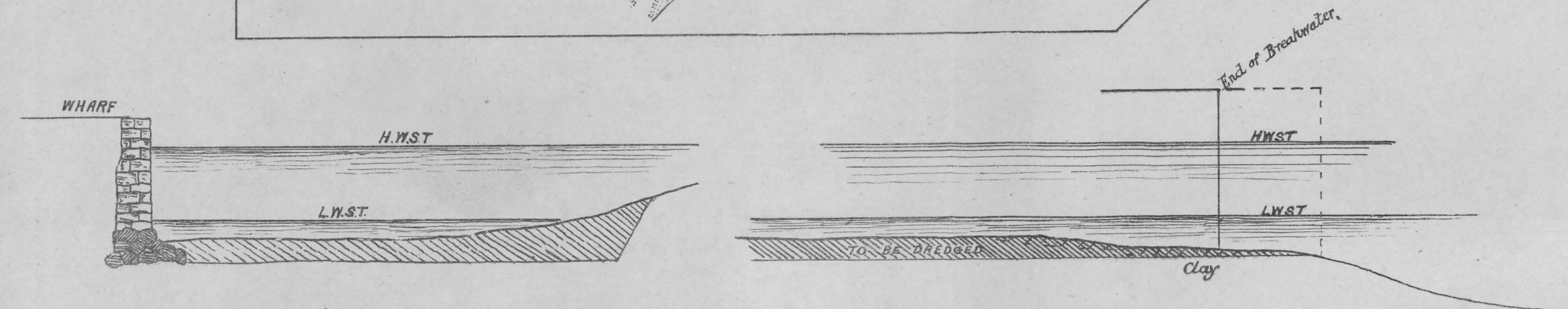
— CROSS SECTION OF CHANNEL — At end of Timber wharf
