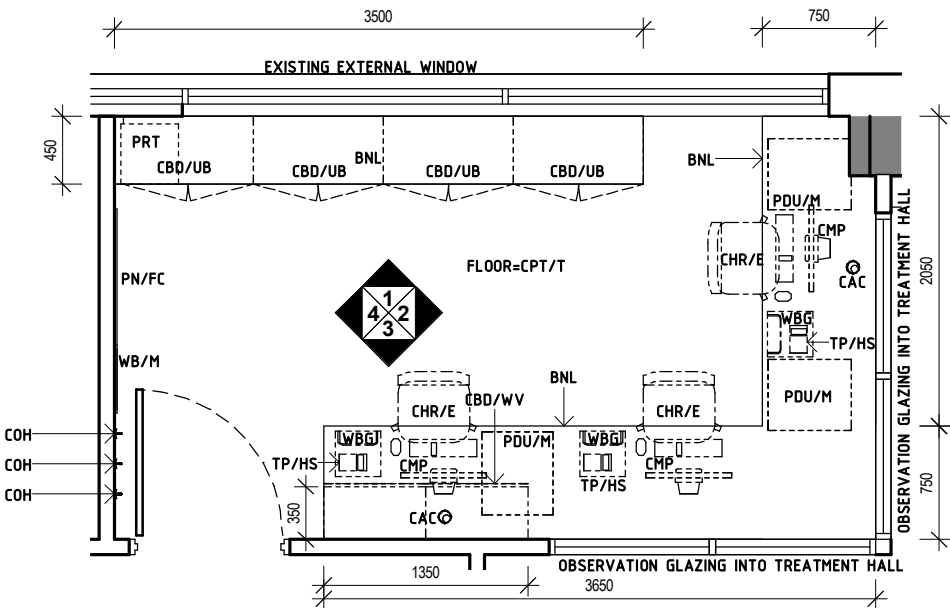
Plan
