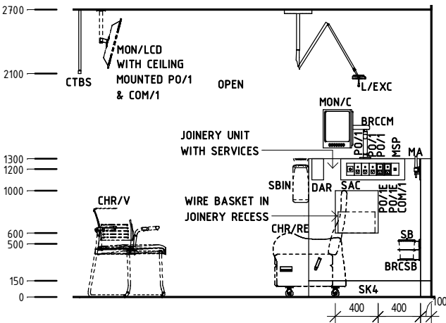
Elevation 3 Elevation 6 Elevation 8 Elevation 11 (mirrored)
