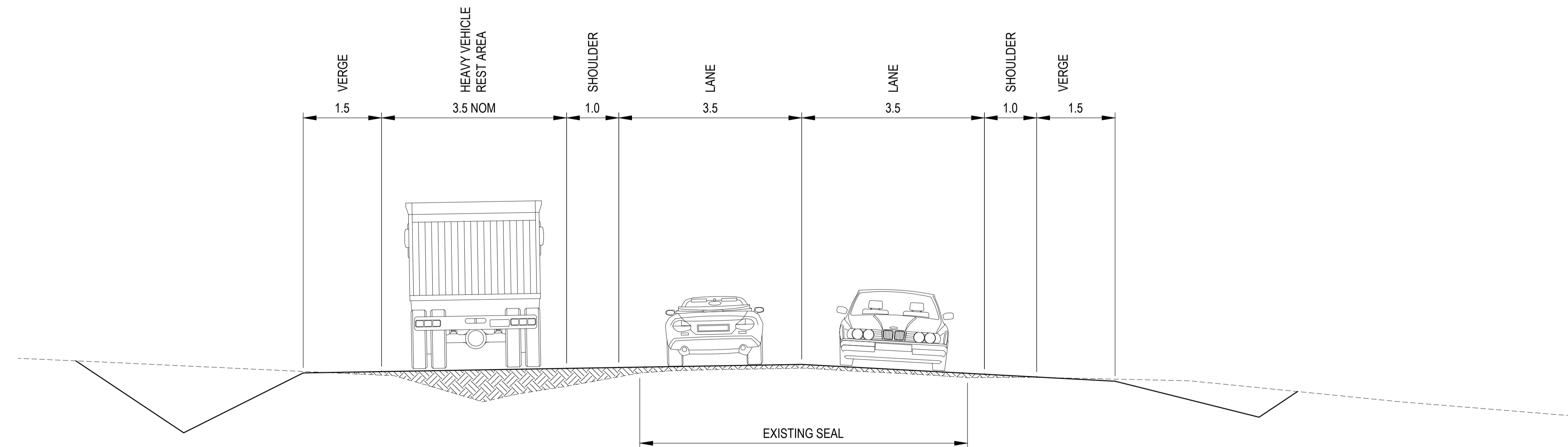
Sidmouth Heavy Vehicle Rest Area (LHS) - Typical Section
