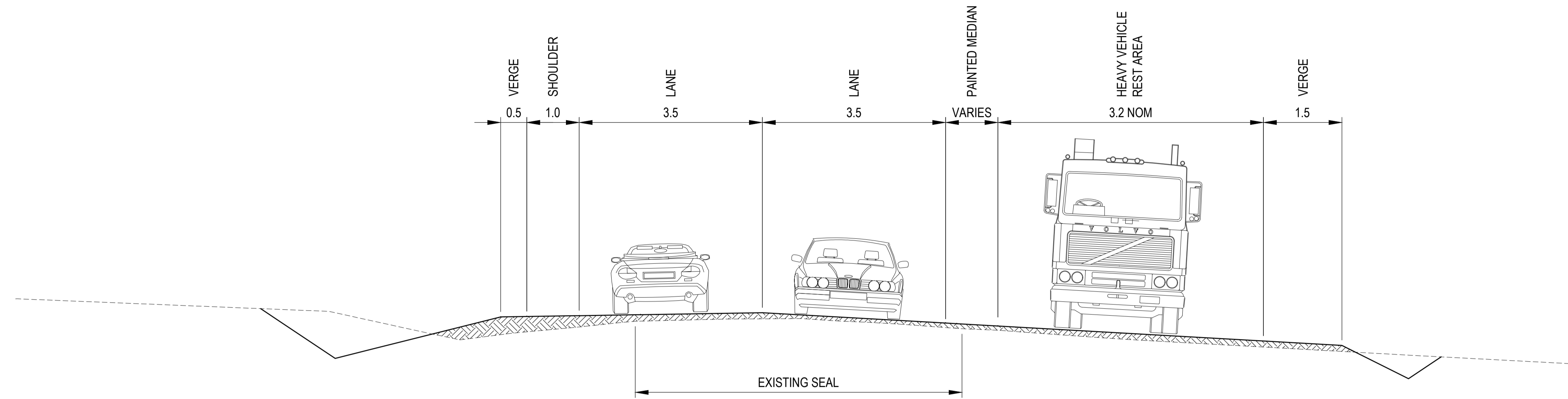
Sidmouth Heavy Vehicle Rest Area (RHS) - Typical Section
