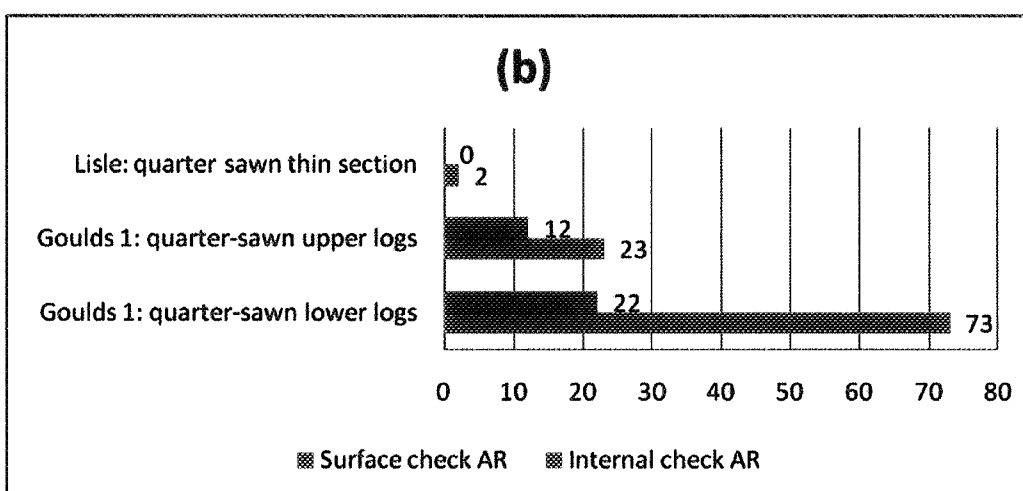
Figure 18a–b. Comparison of the percentage of E. nitens boards with internal and surface checking between studies: AR = after reconditioning; Goulds 1 = Washusen et al. (2007a); Goulds 2 = Blakemore et al. (2010a); Lisle = Blakemore et al. (2010b); Upper and lower log locations refer to the top log and butt log from the lower stem
