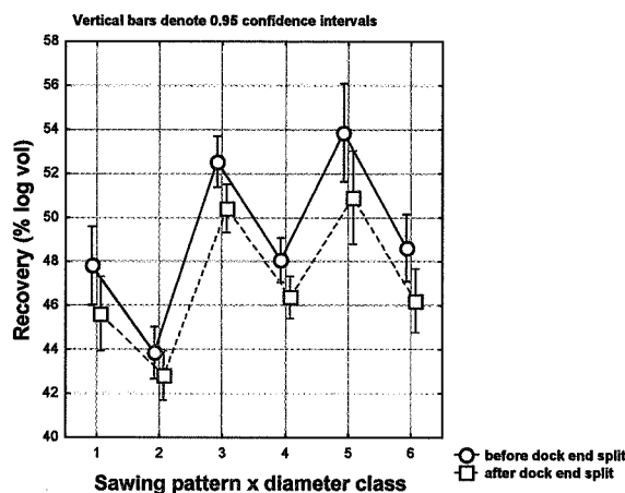
Figure 13. Plot showing loss due in green volume recovery due to end-splits for three different sawing patterns on a HewSaw R250 and two diameter classes for each sawing pattern (Washusen et al. 2007b)
