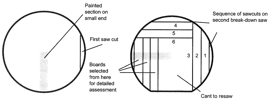
Back-sawing strategy for 30 cm SED log
