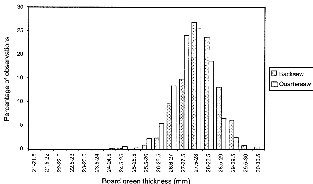
FIGURE 2: Distribution of product thickness measurements for back-sawing and quarter-sawing.
